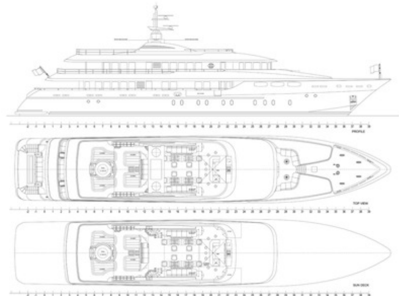
General Arrangement
