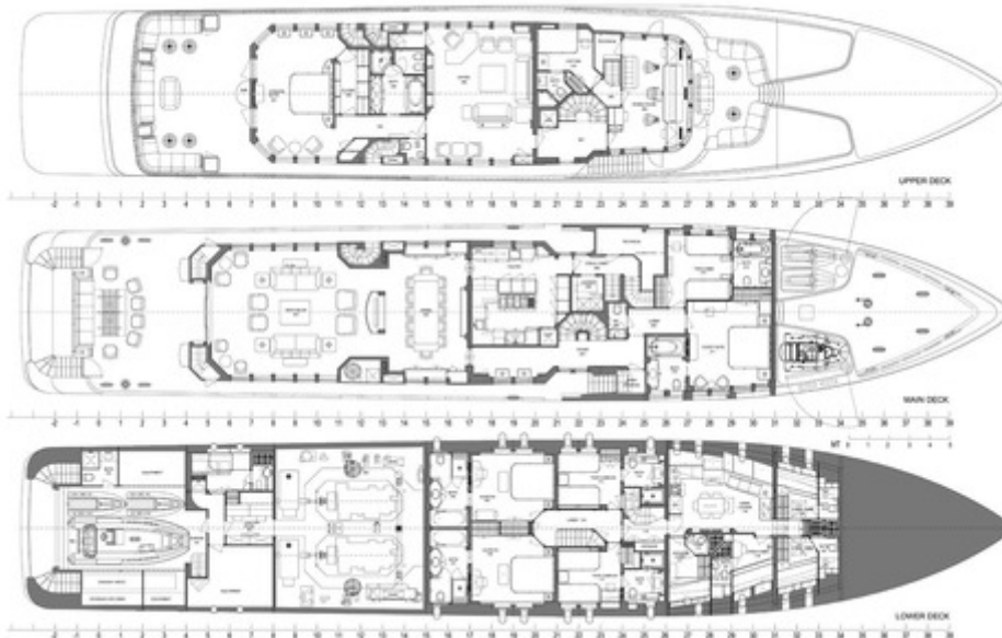
General Arrangement
